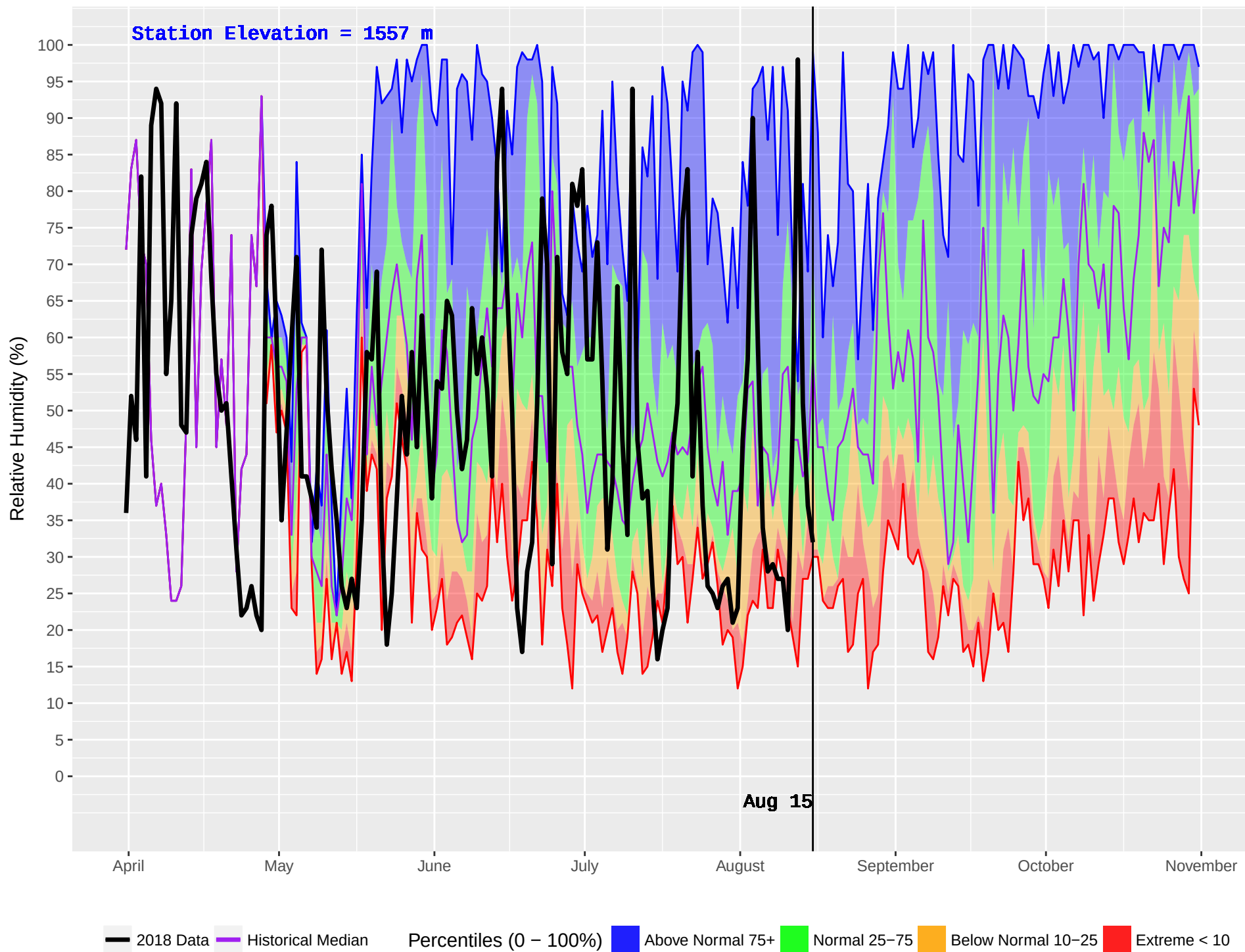
SKOONKA (1024) : Historical (2008–2016) and Current (2018) Daily Relative Humidity
