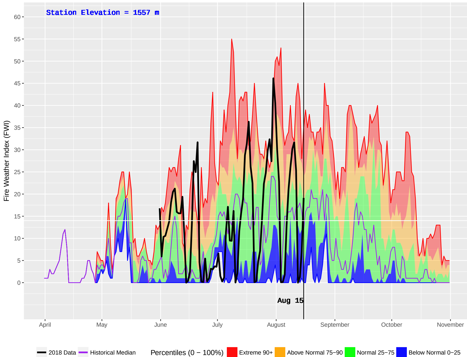
SKOONKA (1024) : Historical (2008–2016) and Current (2018) Daily Fire Weather Index (FWI)
